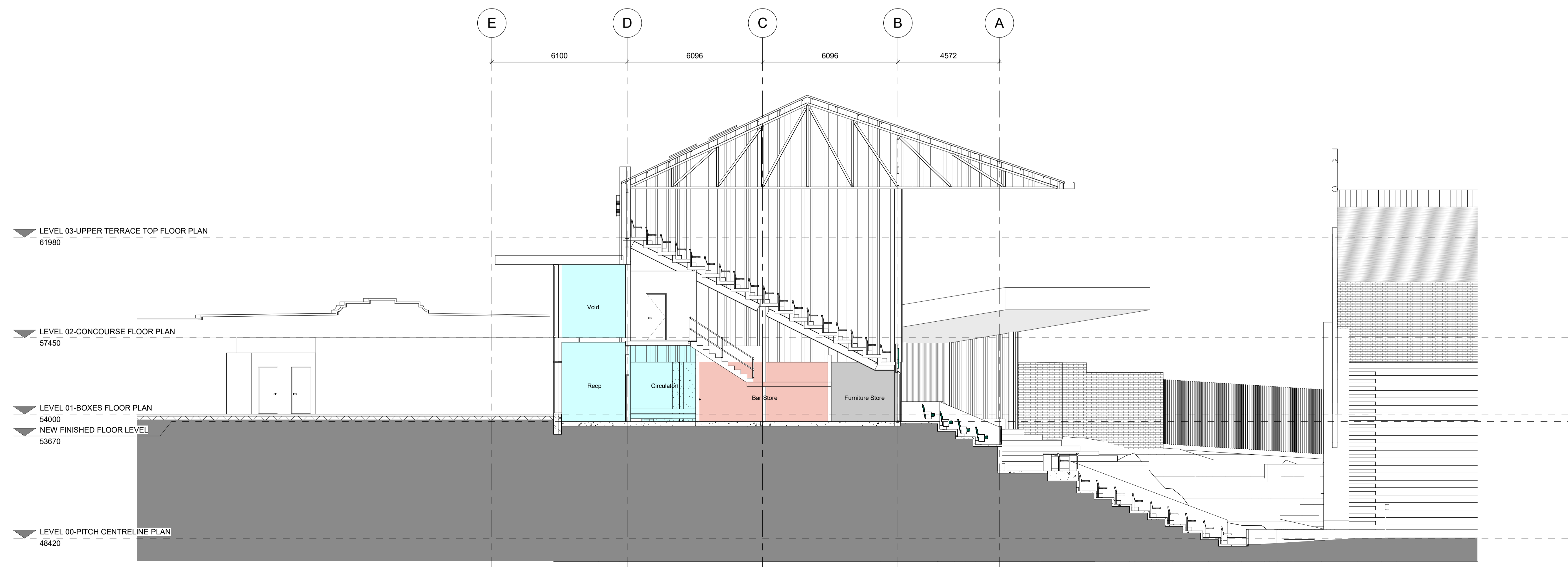
Section 4 Stage 1 1 : 100
