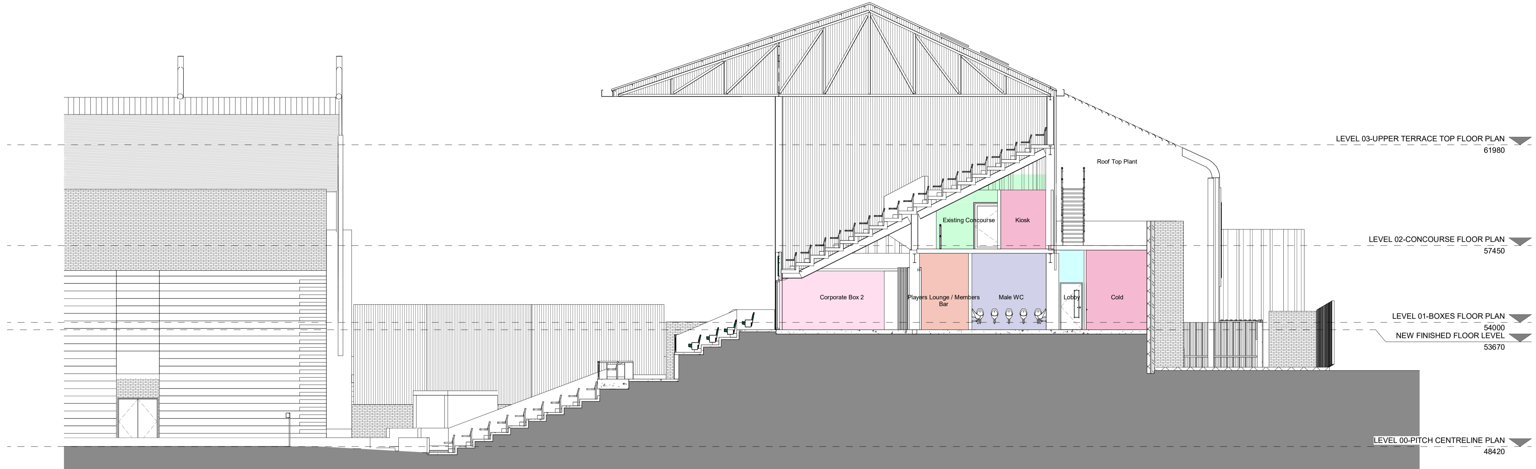
Section 3 Stage 1 1 : 100
