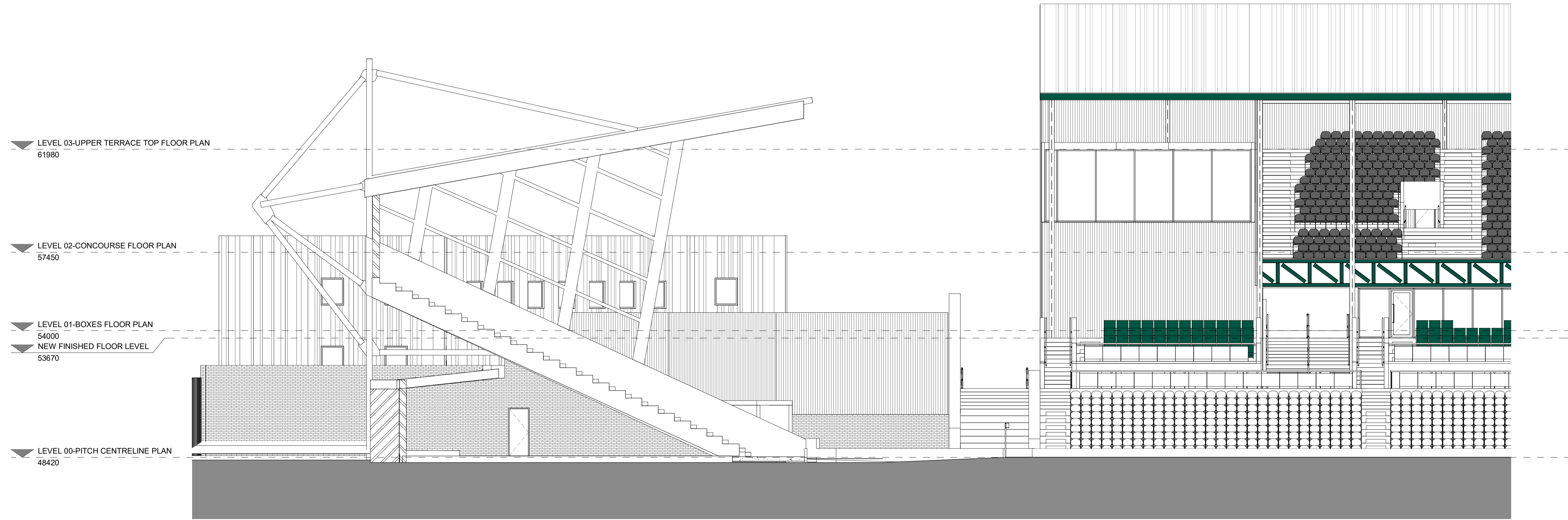
Section 6 Stage 1 1 : 100
