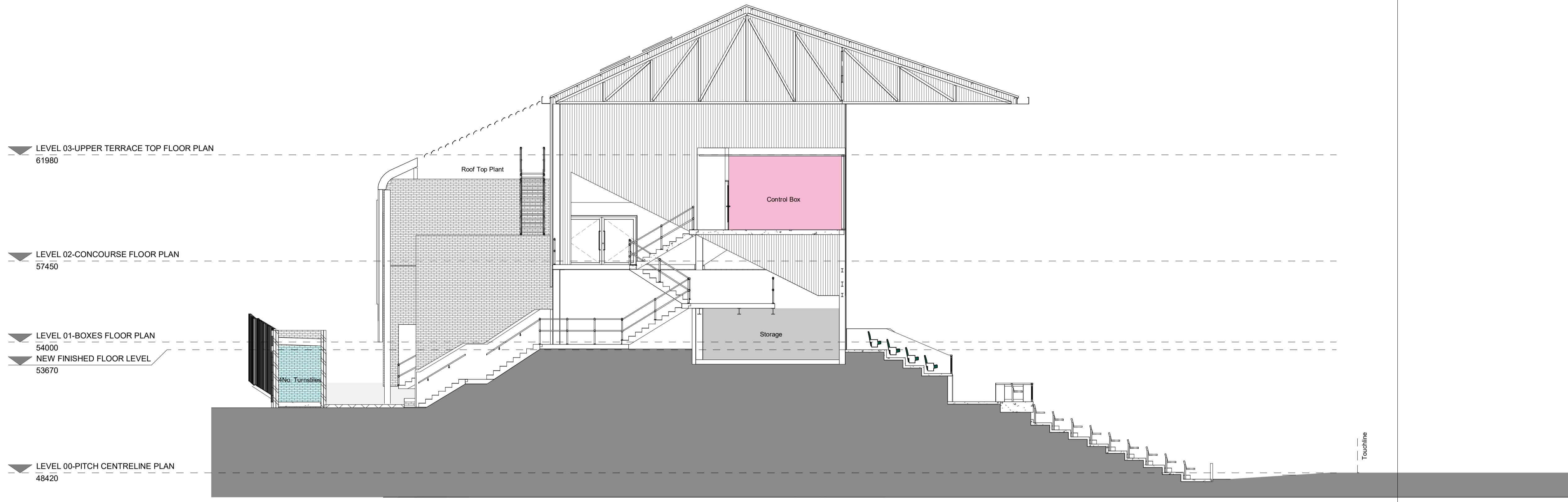
Section 5 Stage 1 1 : 100
